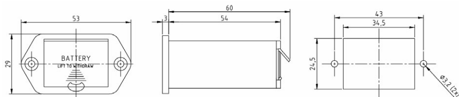
Dimensions of the battery box P/N ST50-65
